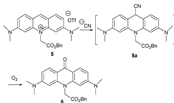
Scheme 3 Proposed mechanism for the reaction-based detection of cyanide ion by indicator 5 .
