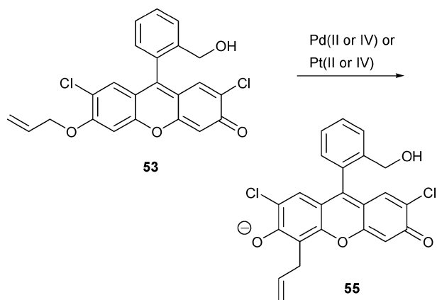
Scheme 24 Additional palladium-dependent reactions of 53 .
