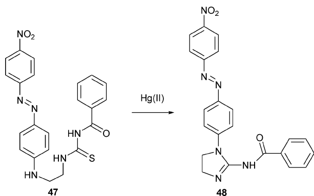
Scheme 20 Proposed mechanism for the reaction-based detection of mercury by indicator 47 .
