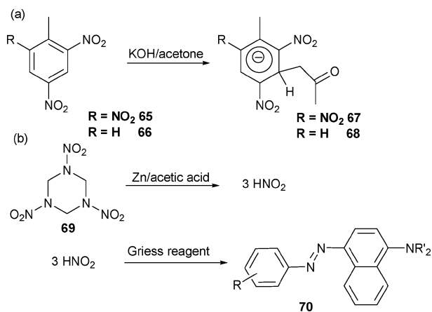
Scheme 29 (a) Reactions of TNT and DNT that have traditionally been used for sensing. (b) Reaction of RDX that has been used for the same purpose.
