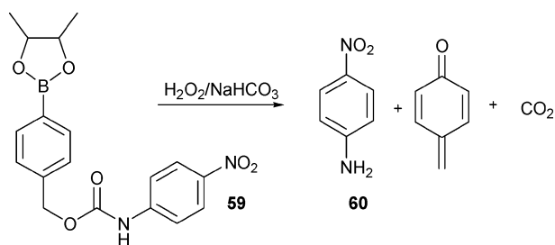
Scheme 26 Hydrogen peroxide-sensing reaction of 59 .
