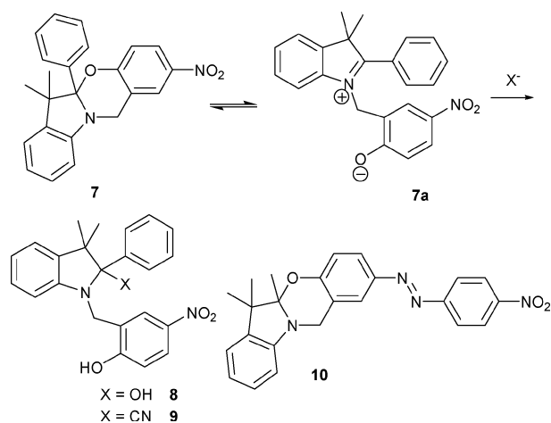
Scheme 4 Proposed mechanism for the reaction-based detection of cyanide ion by indicator 10 .
