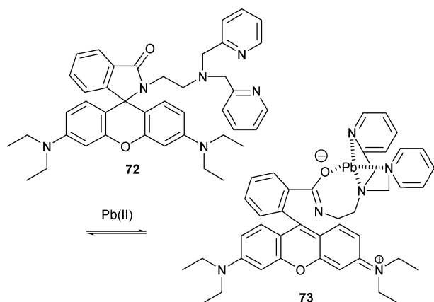
Scheme 31 Proposed lead-sensing mechanism of 72 .
