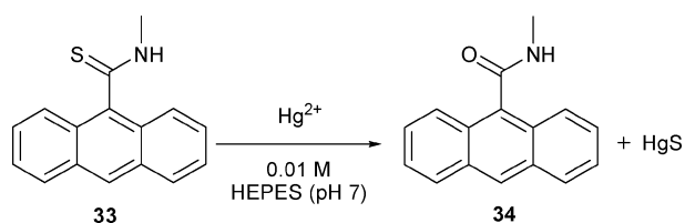
Scheme 13 Proposed mechanism for the reaction-based detection of mercury by indicator 33 .
