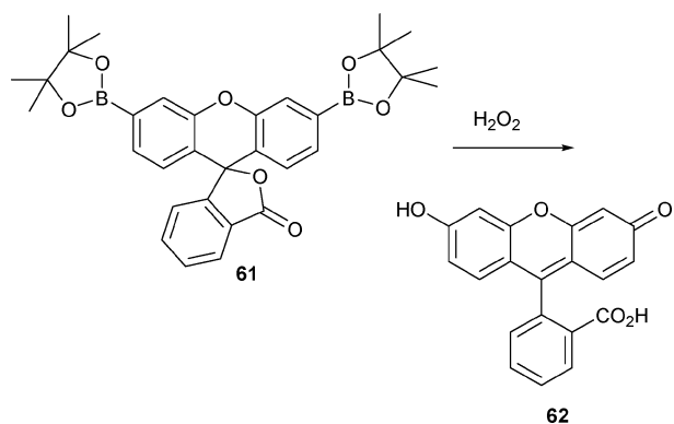
Scheme 27 Hydrogen peroxide-sensing reaction of 61 .
