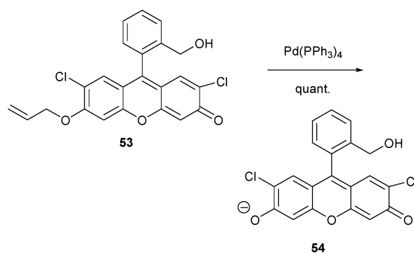
Scheme 23 Palladium-dependent reactions of 53 .
