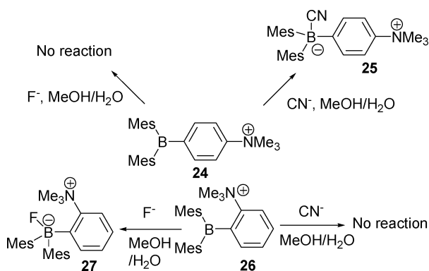
Scheme 11 Cyanide- and fluoride-sensing reactions of indicators 24 and 26 .
