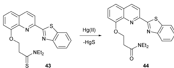
Scheme 18 Proposed mechanism for the reaction-based detection of mercury by indicator 43 .
