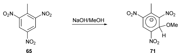
Scheme 30 A reaction used to detect the presence of TNT.
