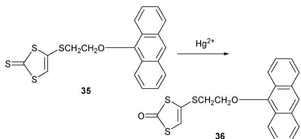
Scheme 14 Proposed mercury-sensing mechanism of 35 .
