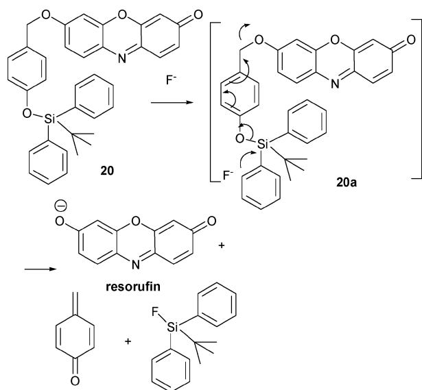
Scheme 9 Proposed mechanism for the reaction-based detection of fluoride by indicator 20 .
