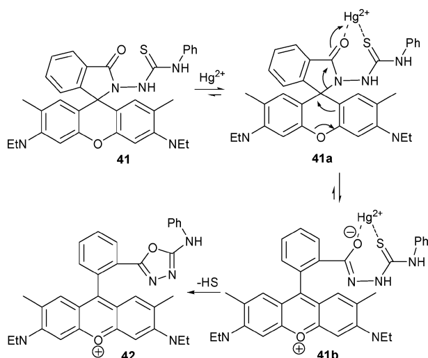
Scheme 17 Proposed mechanism for the reaction-based detection of mercury by indicator 41 .
