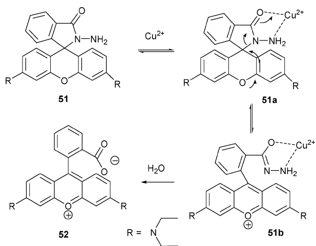
Scheme 22 Proposed copper(II)-based reactions considered relevant to an understanding of indicator 51 .
