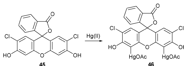
Scheme 19 Proposed mechanism for the reaction-based detection of mercury by indicator 45 .
