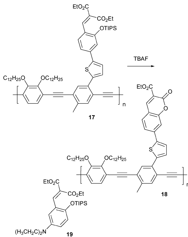
Scheme 8 Proposed mechanism for the reaction-based detection of fluoride by indicator 17 .
