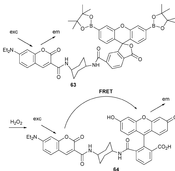
Scheme 28 Hydrogen peroxide-induced transformation of indicator 63 into product 64 and the FRET pathway expected in the latter species.
