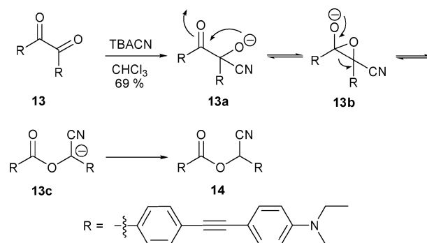
Scheme 6 Proposed mechanism for the reaction-based detection of cyanide ion by indicator 13 .
