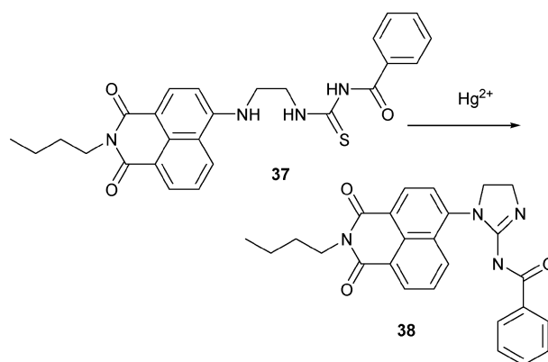
Scheme 15 Proposed mechanism for the reaction-based detection of mercury by indicator 37 .
