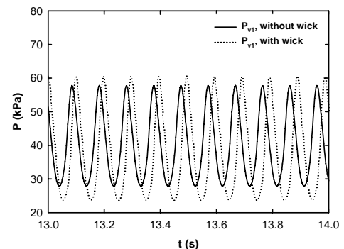
(c) Vapor plug pressure
