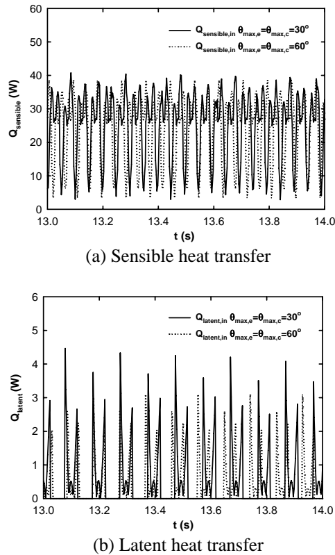
Fig. 6 Effect of \theta_{\max,e} and \theta_{\max,c} on sensible and evaporative heat transfer with wick
