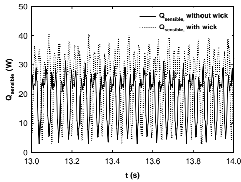
(a) Sensible heat transfer
