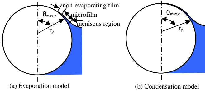
Fig. 2 Evaporation and condensation occurred on sintered particles
