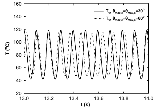
(b) Vapor plug temperature
