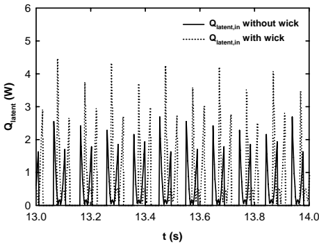
(b) Latent heat transfer
