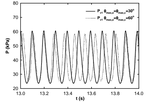
(c) Vapor plug pressures
