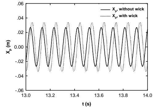
(a) Displacement of liquid slug
