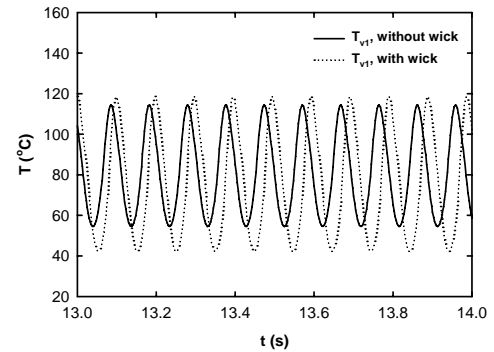
(b) Vapor plug temperatures
