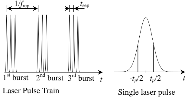
Fig. 2 Laser pulse train
