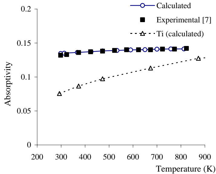
Figure 5. Temperature-dependent Absorptivity for Titanium Alloy Ti-6Al-4V (10.6 μm).
